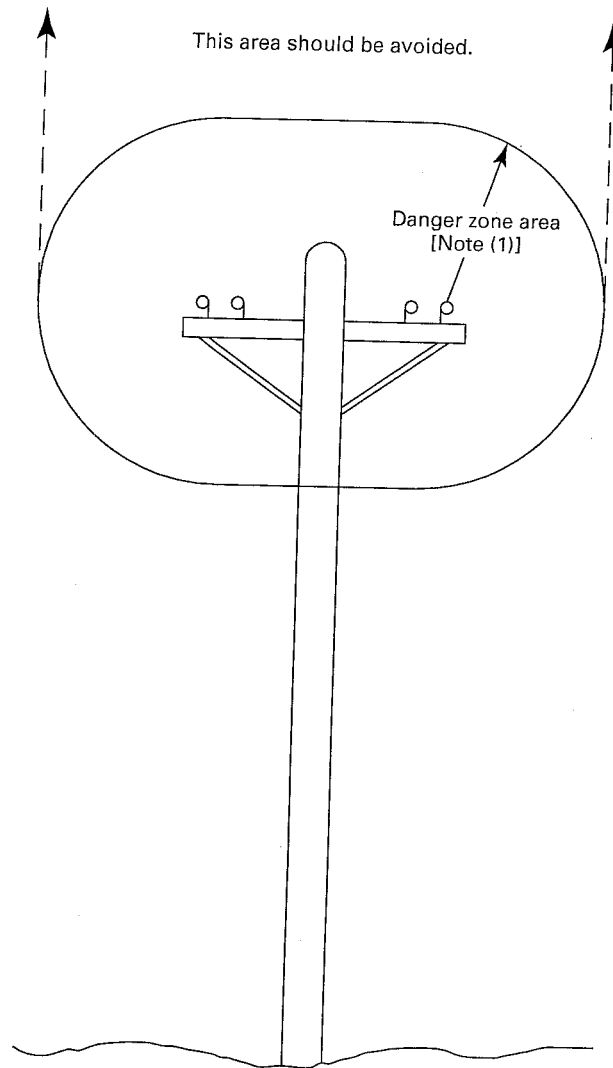
Fig. 8-3.4.3-1 Danger Zone for Cranes, Derricks, and Lifted Loads Operating Near Electrical Transmission Lines
