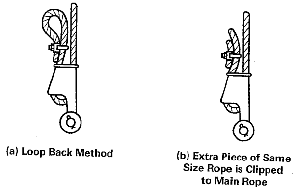
Fig. 8-1.9.3-1 Dead Ending Rope in a Socket
