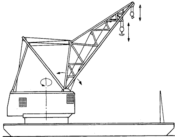
Fig. 8-0.1-1 Floating Crane
