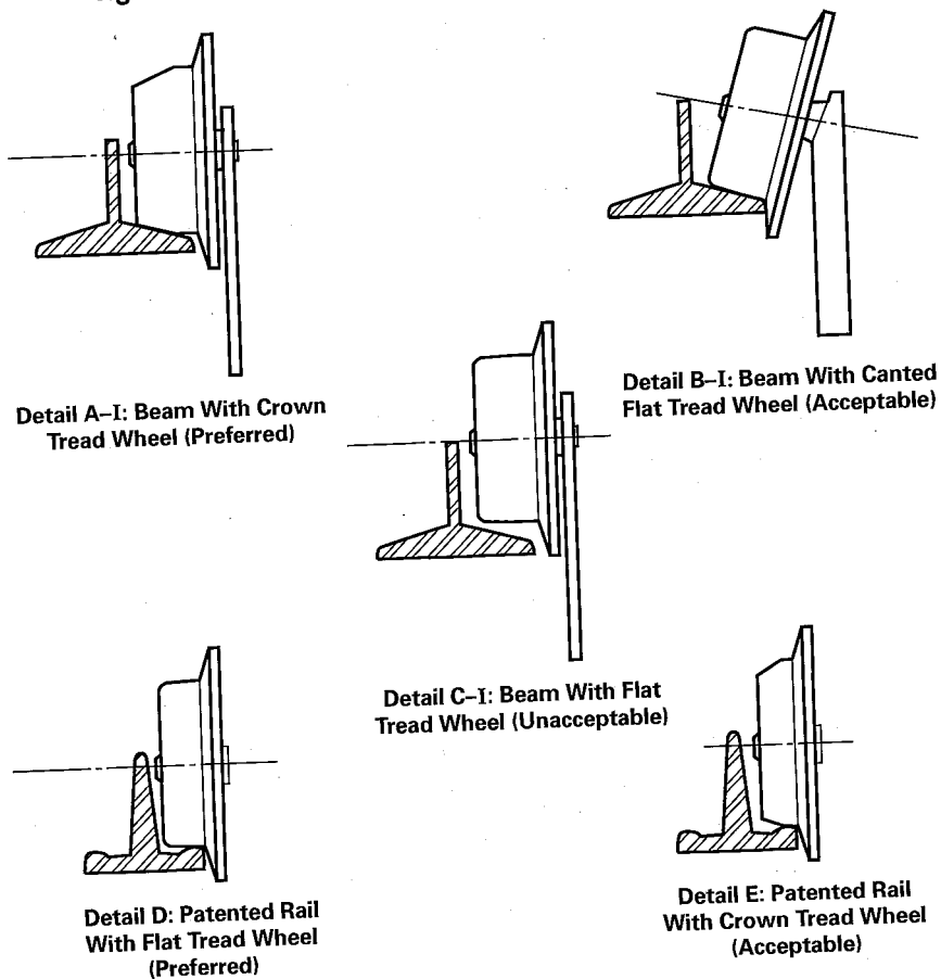
Fig. 11-1.13-1 Recommended Trolley Wheel Configurations
