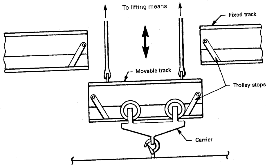
Fig. 11-0.2-6 Drop Section (Lift Section)
