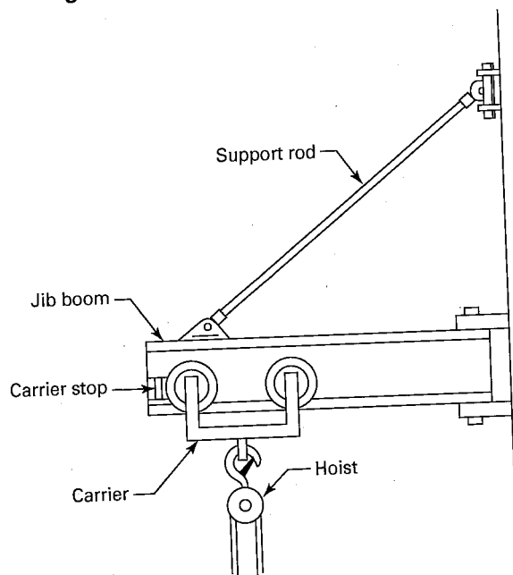
Fig. 11-0.2-8 Wall-Supported Jib Crane
