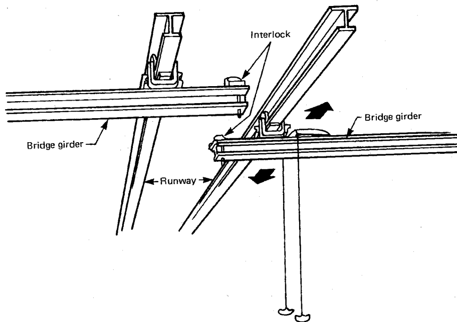
Fig. 11-0.2-7 Interlocking System for Underhung Crane
