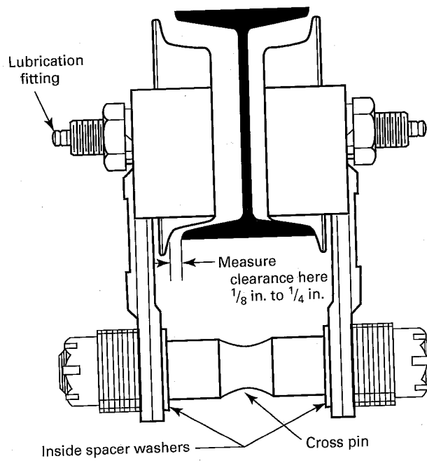
Spacer Washer Arrangement (Minimum Flange Width Shown)
