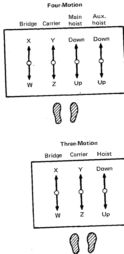
Fig. 11-1.9.3-4 Recommended Arrangement of Controllers (Radio Crane Control Transmitter Lever Arrangement)
