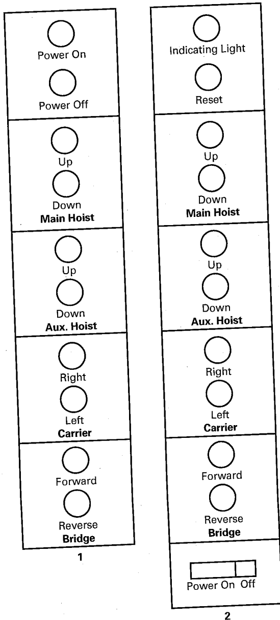
Fig. 11-1.9.3-3 Recommended Arrangement of Controllers (Pendant Push-Button Station Arrangement)
