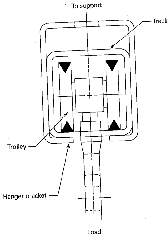
Fig. 11-0.2-9 Example of One Type of Enclosed Track and Support Bracket
