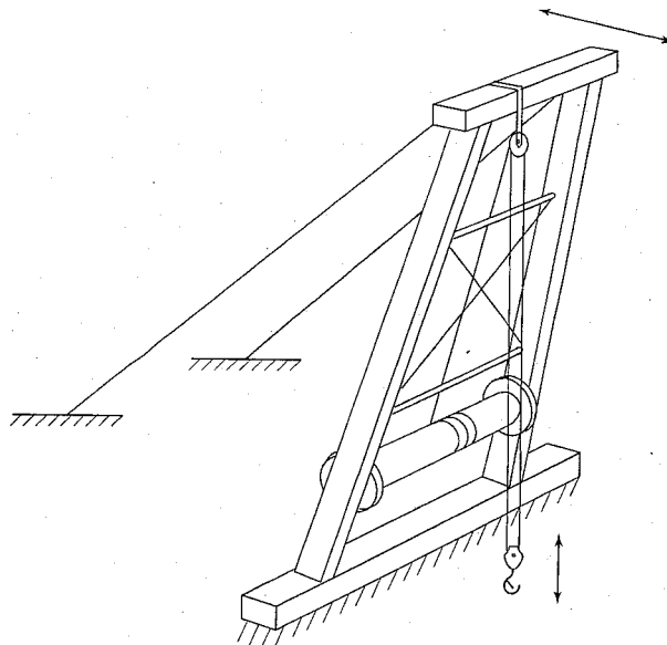
Fig. 6-0.2.1-3 Breast Derrick
