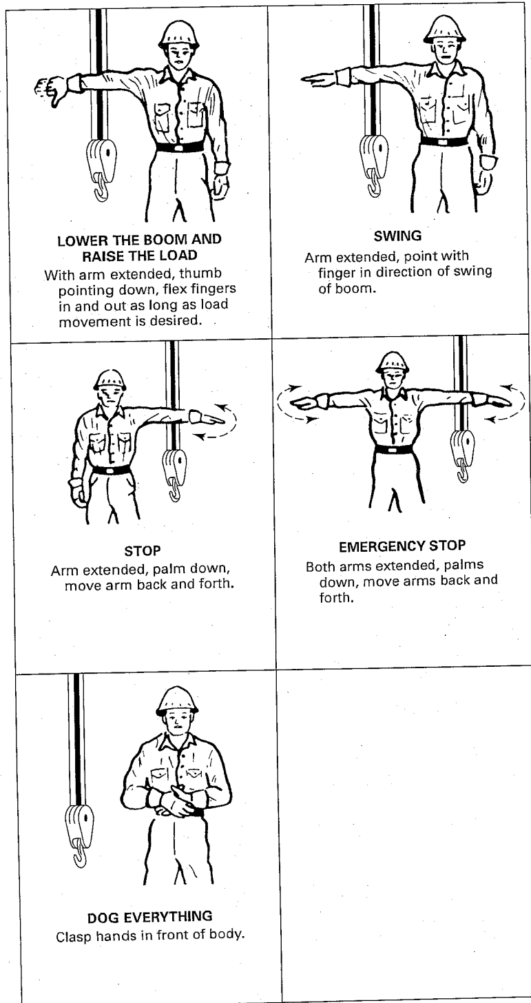
Fig. 6-3.4.2-1 Standard Hand Signals for Controlling Derricks (Cont'd)
