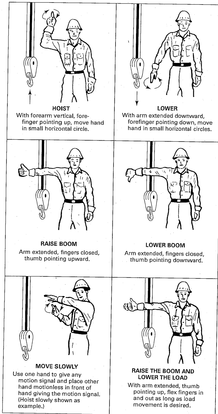
Fig. 6-3.4.2-1 Standard Hand Signals for Controlling Derricks
