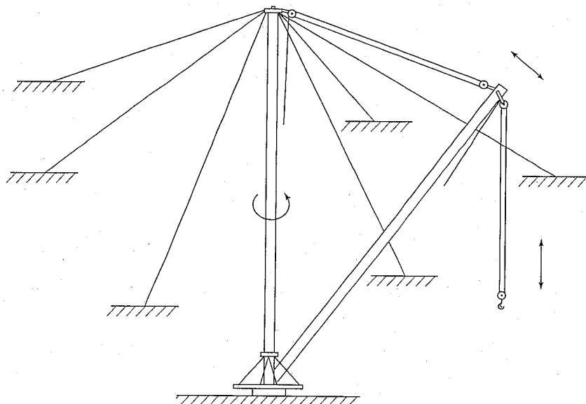
Fig. 6-0.2.1-6 Guy Derrick
